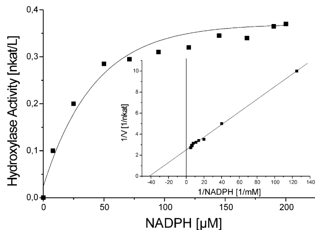
Figure 2. The effect of NADPH concentration on deoxysarpagine hydroxylase activity (standard incubation mixture, K_m = 25 \mu\text{M} , V_{\max} = 0.36 \text{ nkat} ). The insert shows the double-reciprocal plot.
