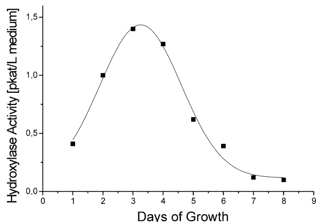
Figure 1. Changes of deoxysarpagine hydroxylase activity of R. serpentina cell cultures during a cultivation period of 8 days.
