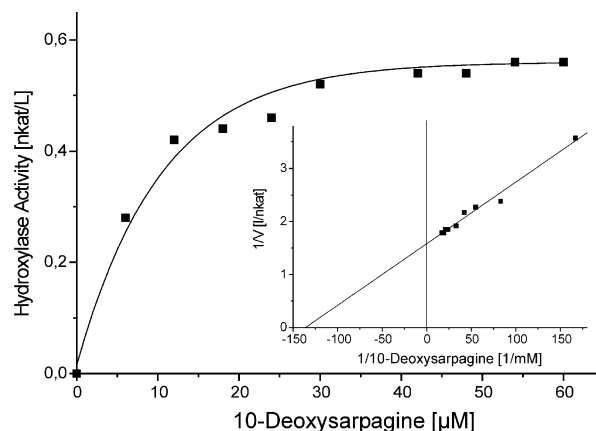
Figure 3. The effect of 10-deoxysarpagine concentration on deoxysarpagine hydroxylase activity (standard incubation mixture, K_m = 7.4 \mu\text{M} , V_{\max} = 0.55 \text{ nkat} ). The insert shows the double-reciprocal plot.
