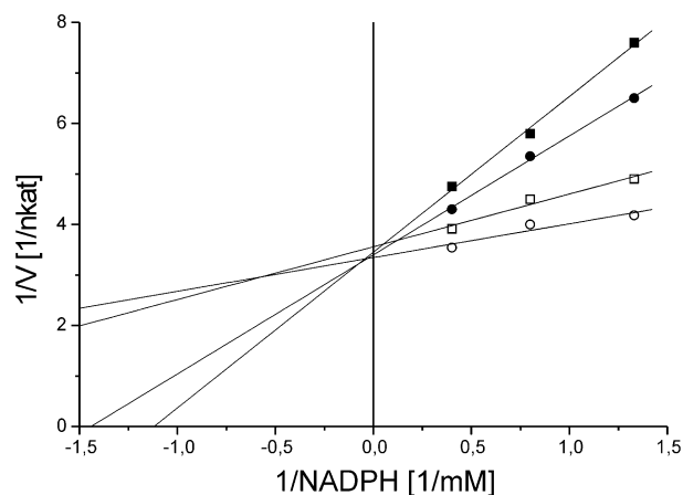
Figure 4. Competitive inhibition of deoxysarpagine hydroxylase by \text{NADP}^+ in presence of 0.75, 1.25, 2.5 mM NADPH (Lineweaver-Burk plot: \circ , without \text{NADP}^+ ; \square , 0.5 mM \text{NADP}^+ ; \bullet , 1.0 mM \text{NADP}^+ ; \blacksquare , 1.5 mM \text{NADP}^+ ).
