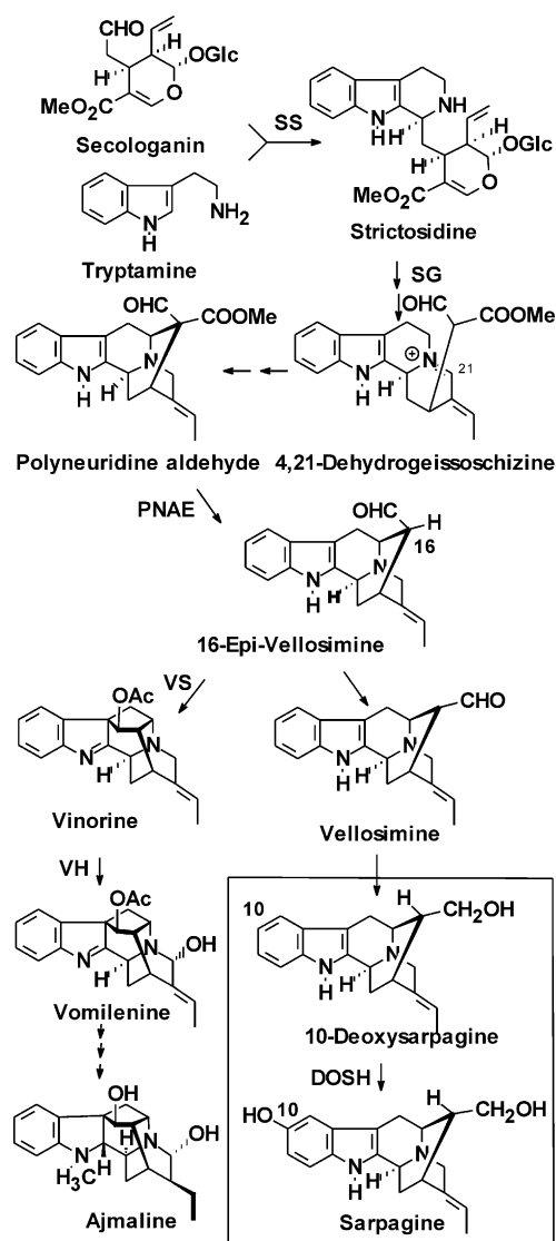
Scheme 1. Major steps of the biosynthetic pathways of sarpagine- and ajmalan-type alkaloids in cell suspension culture of Rauvolfia serpentina . The reaction catalyzed by the deoxysarpagine hydroxylase (hydroxylation to sarpagine at carbon position 10) is boxed (DOSH, deoxysarpagine hydroxylase; PNAE, polyneuridine aldehyde esterase; SG, strictosidine glucosidase; SS, strictosidine synthase; VH, vinorine hydroxylase; VS, vinorine synthase).
